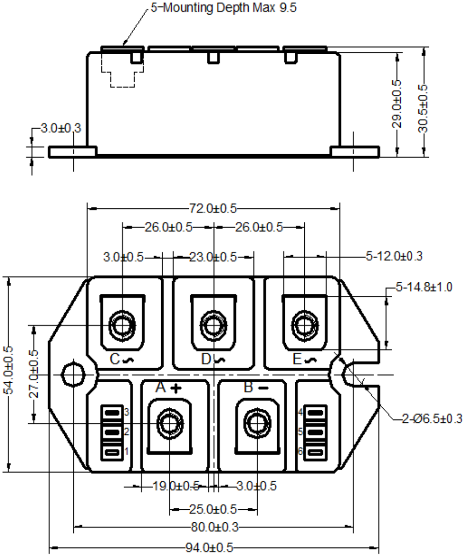
Dimensions in (mm) Figure 6. Package Outline
