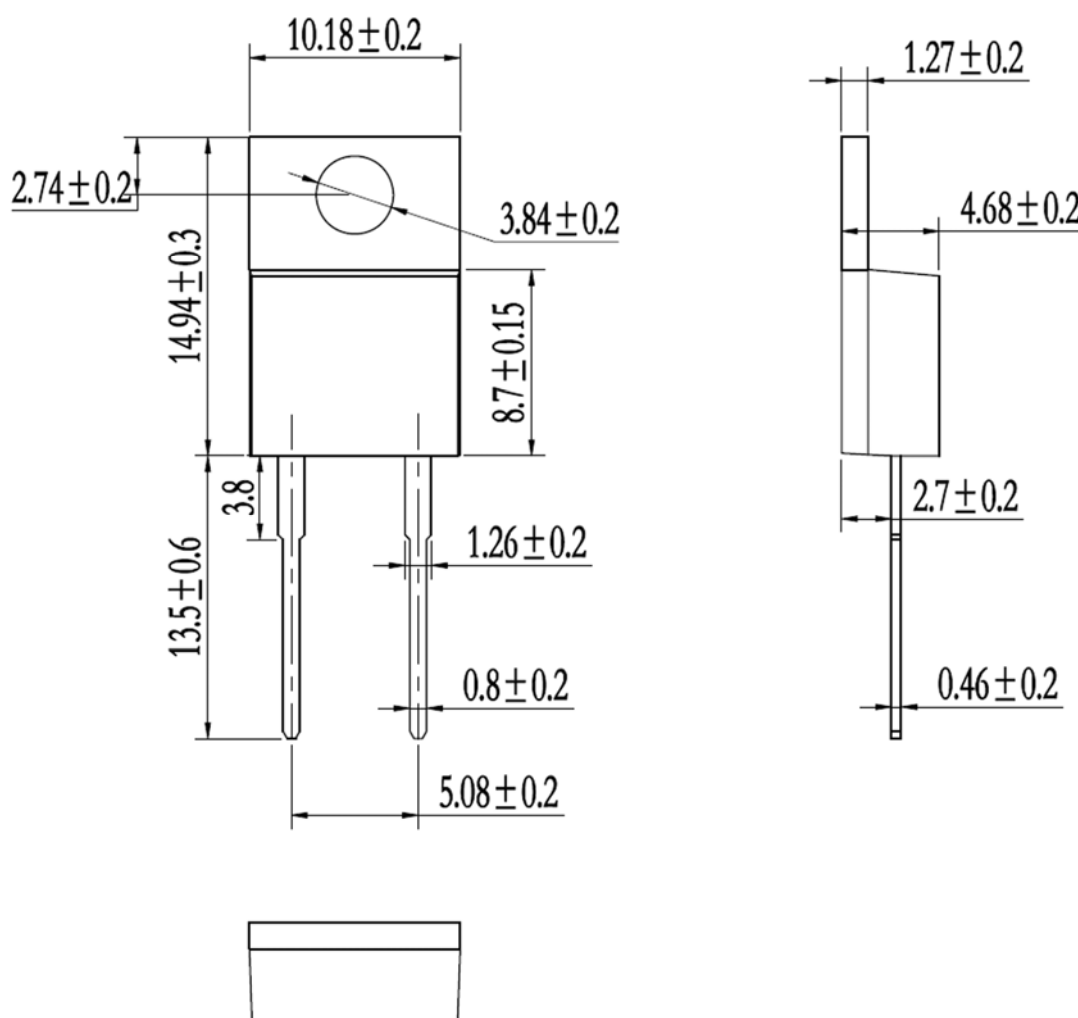
Dimensions in Millimeters Figure8. Package Outline
