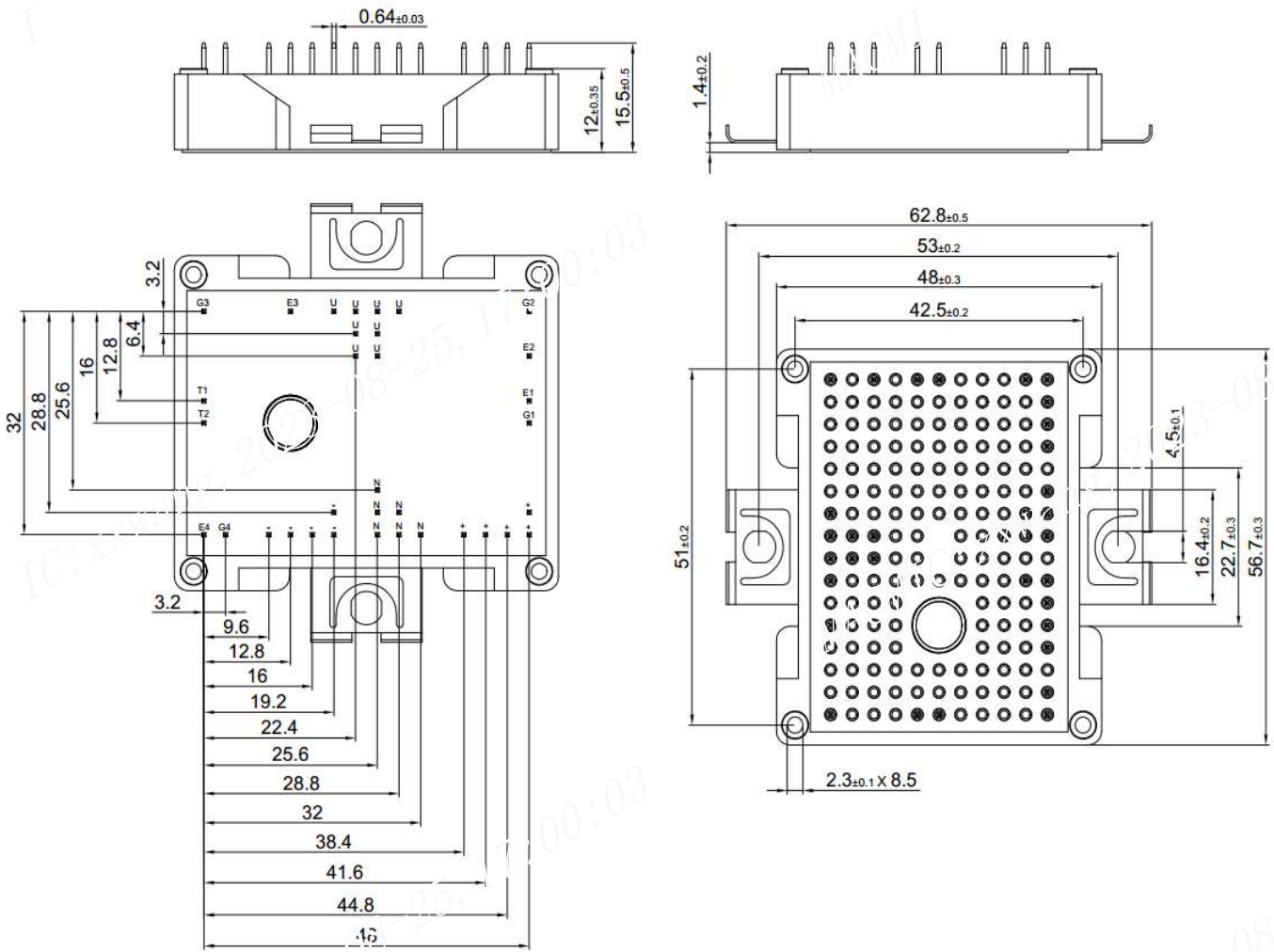
Dimensions in (mm) Figure 15. Package Outline
