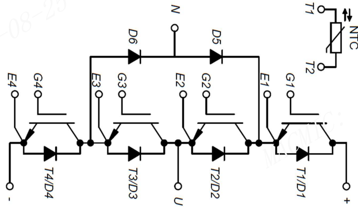
Figure 14. Circuit Diagram
