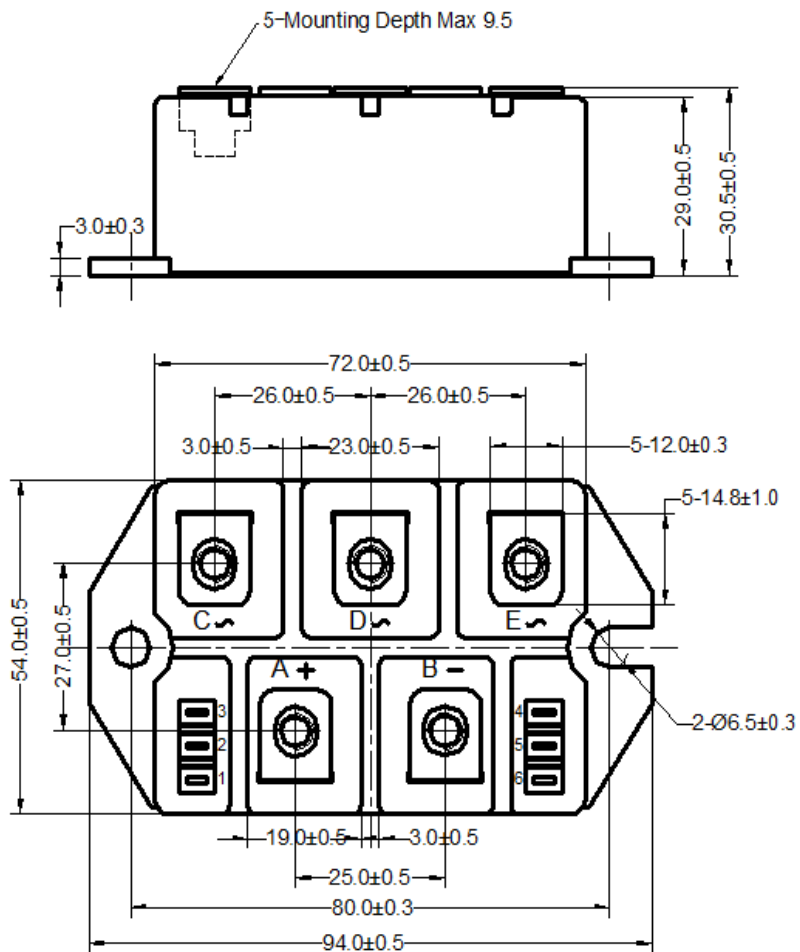
Figure 6. Package Outline
