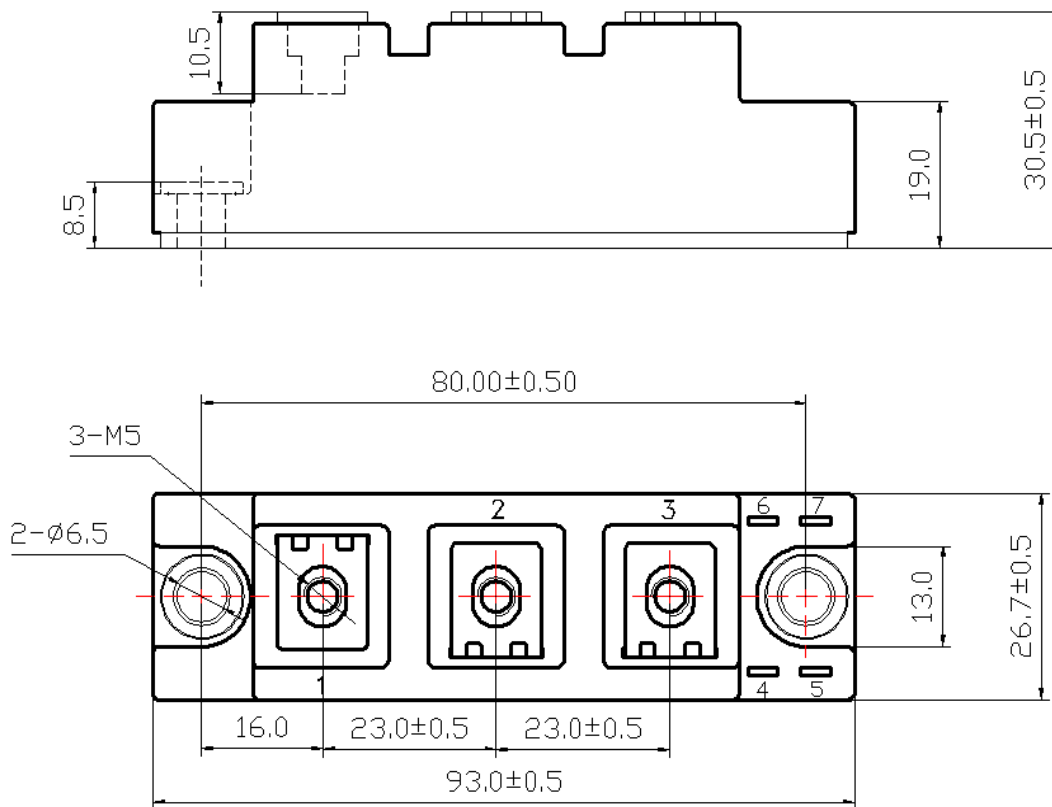
Dimensions in (mm) Figure 6. Package Outline
